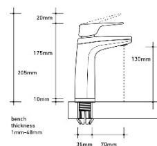
XL Levered tap dimensions
